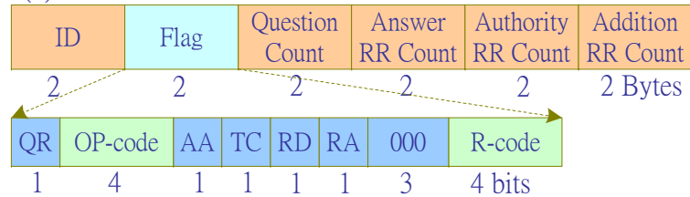
(b) DNS Header
