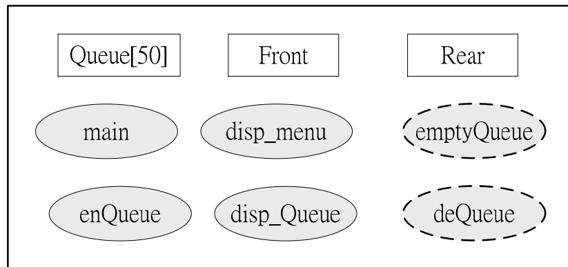
PM4_4.java (PM4_4.class)
